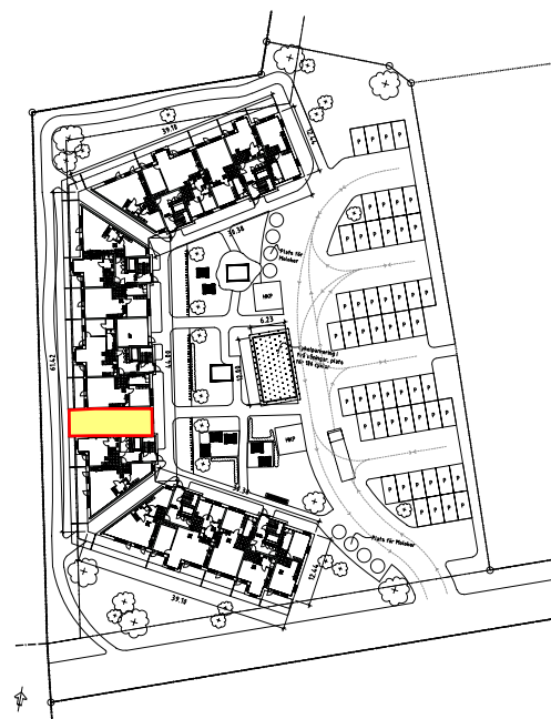
Situationsplan
